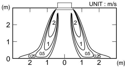
SIDE VIEW AIR FLOW DIRECTION : Downward
