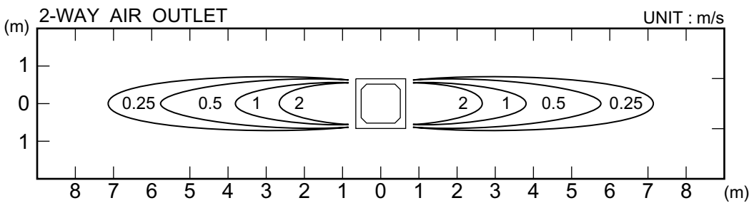
TOP VIEW AIR FLOW DIRECTION : Upward
