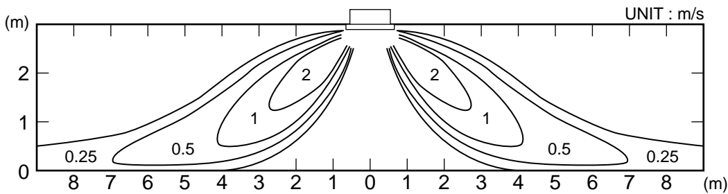
SIDE VIEW AIR FLOW DIRECTION : Upward
