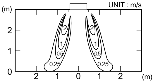
SIDE VIEW HORIZONTAL LOUVER : Downward
