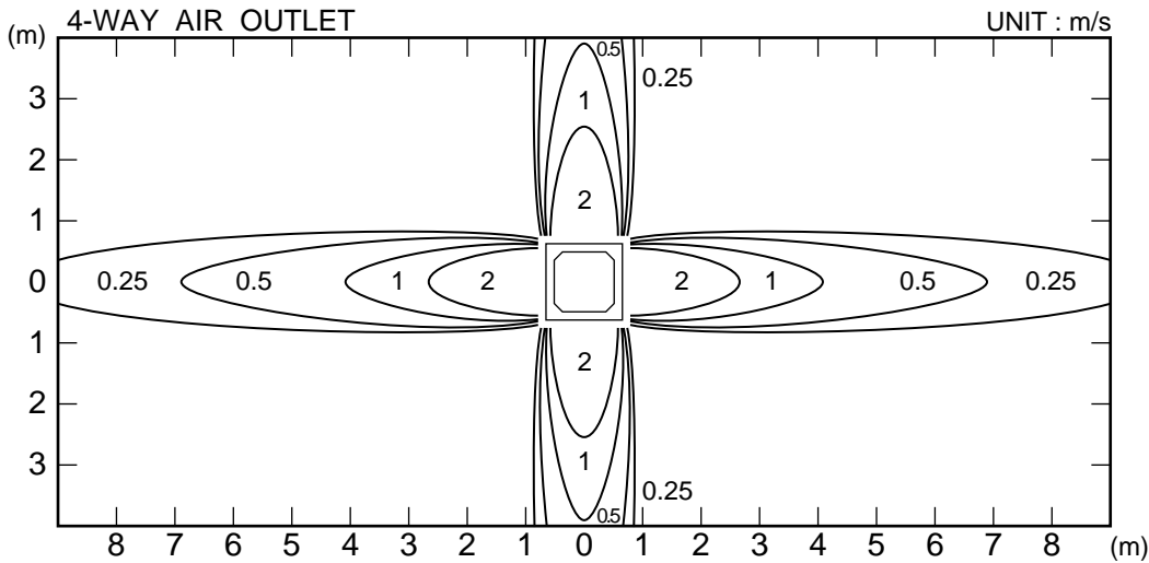
TOP VIEW AIR FLOW DIRECTION : Upward
